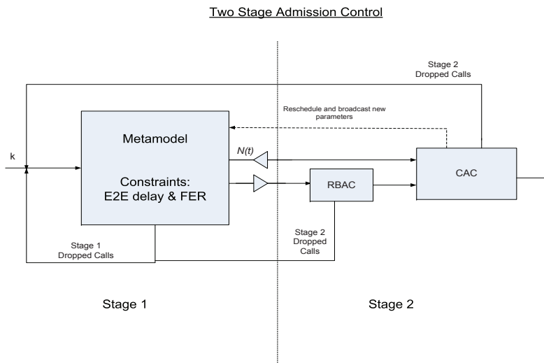
Figure 7: Two Stage Admission Control Modular Design
