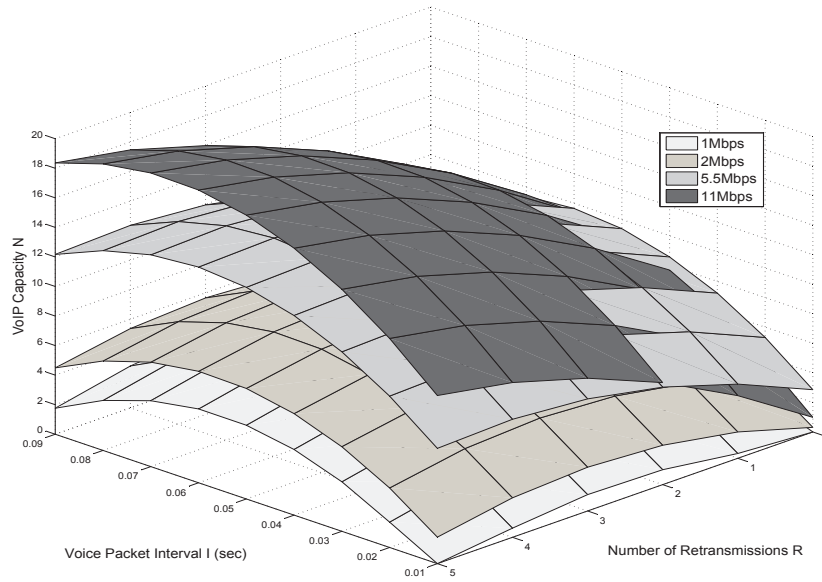
Figure 4: VoIP call capacity ( N ) for PER = 10^{-5}
