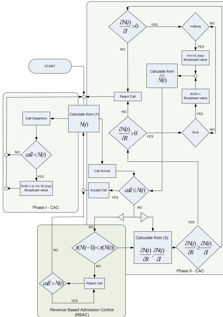
Figure 8: Flow chart of the algorithm: Optimal Capacity Allocator with a separate module for RBAC
