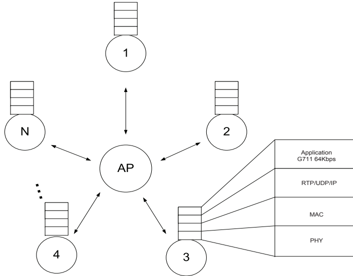
Figure 1: Simulation scenario of the layered network.
