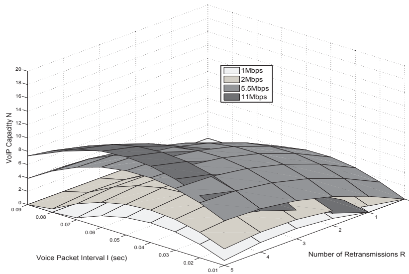
Figure 5: VoIP call capacity ( N ) for PER = 10^{-1}
