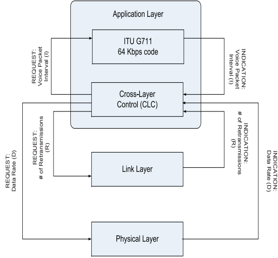
Figure 2: Cross-Layer Control (CLC) module and cross-layer interactions.
