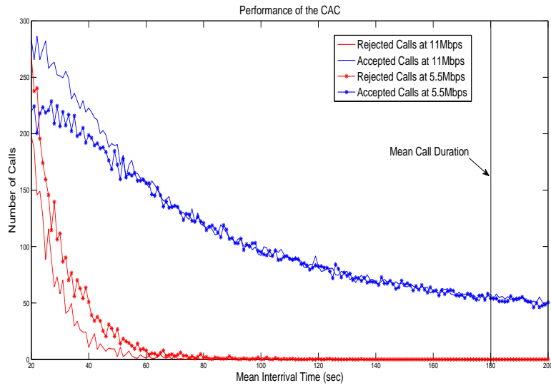
Figure 9: Performance of the system as a function of mean interarrival time
