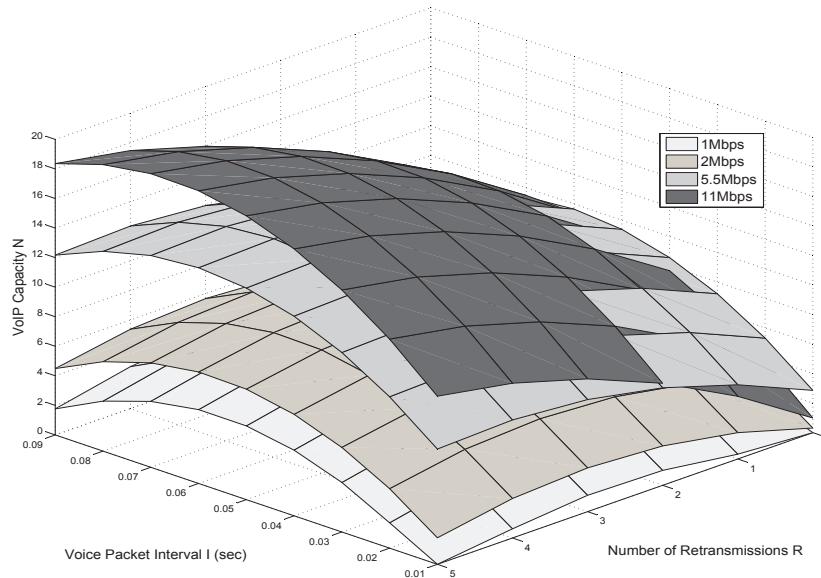
Figure 3: VoIP call capacity ( N ) for PER = 10^{-9}
