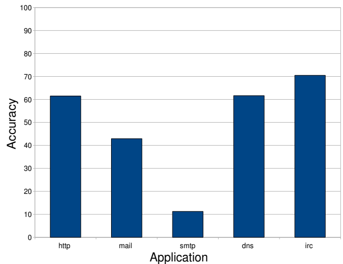
Fig. 2. Accuracy for K-mean clustering and rule-based classification
